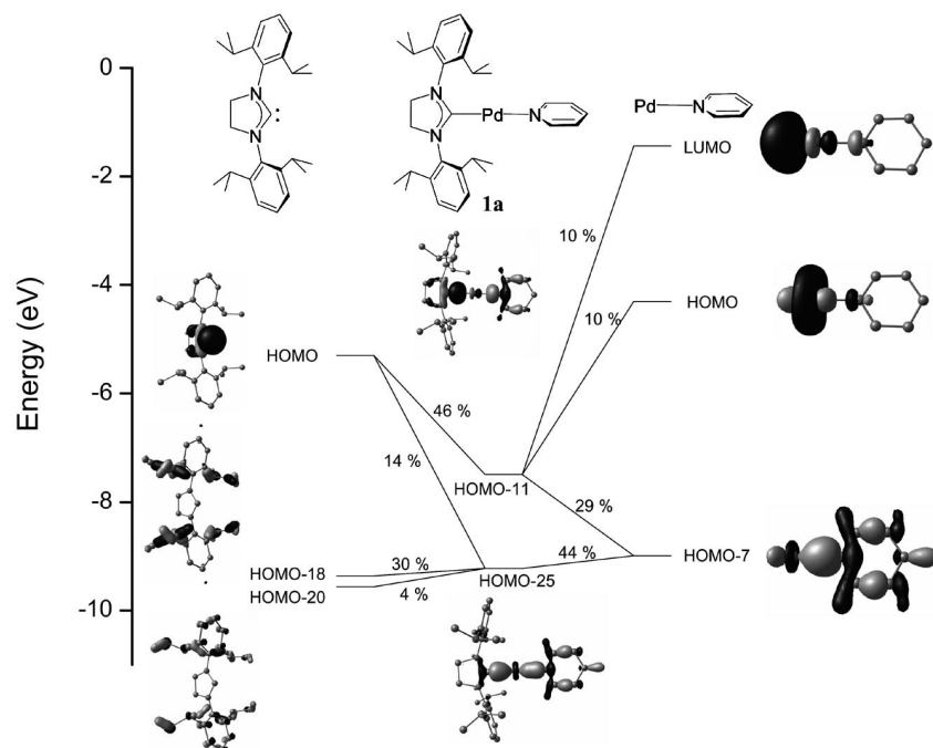
Figure 4. Orbital interaction diagram showing the major contributions of the NHC–palladium bond in 1a .
