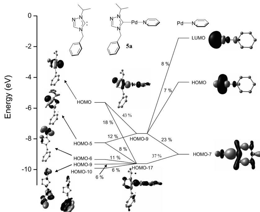
Figure 5. Orbital interaction diagram showing the major contributions of the NHC–palladium bond in 5a .
