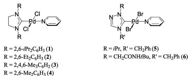
Figure 1. PEPPSI-themed (NHC)PdX 2 (pyridine) (X = halide) complexes of the C4–C5 saturated imidazole- (1–4) and triazole-based (5 and 6) N -heterocyclic carbenes.
