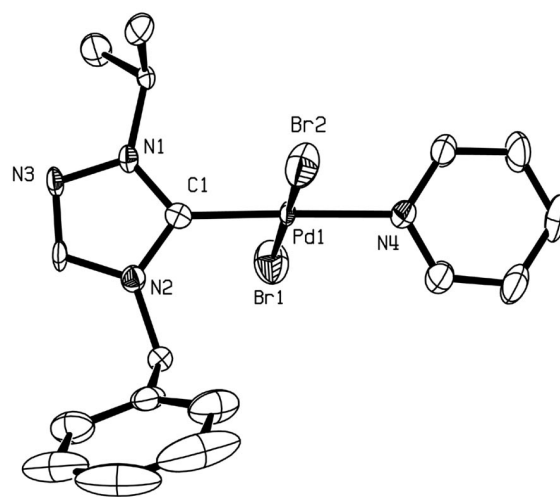
Figure 3. ORTEP drawing of 5 with thermal ellipsoids shown at the 50% probability level. Selected bond lengths [Å] and angles [°]: N(1)–C(1) 1.341(12), N(2)–C(1) 1.375(12), Pd(1)–C(1) 1.950(9), Pd(1)–Br(1) 2.3669(15), Pd(1)–N(4) 2.092(8), C(1)–Pd(1)–N(4) 178.6(3), C(1)–Pd(1)–Br(1) 88.5(3).
