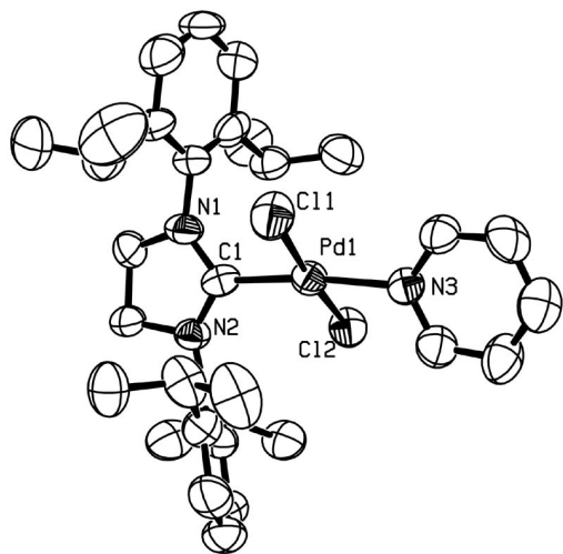
Figure 2. ORTEP drawing of 1 with thermal ellipsoids shown at the 50% probability level. Selected bond lengths [Å] and angles [°]: N(1)–C(1) 1.334(9), N(2)–C(1) 1.317(9), Pd(1)–C(1) 1.993(7), Pd(1)–Cl(1) 2.294(2), Pd(1)–N(3) 2.106(6), C(1)–Pd(1)–N(3) 174.2(3), C(1)–Pd(1)–Cl(1) 93.7(2).
